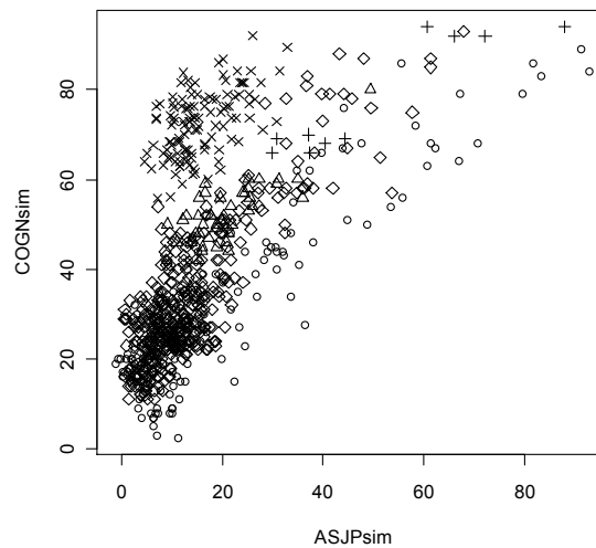
Figure 1. Scatter-plot of COGNsim as a function of ASJPsim for individual language pairs pertaining to five selected families: Australian (o), Uto-Aztecan ( \diamond ), Japonic (+), Carib ( \Delta ), Sino-Tibetan ( \times ).
