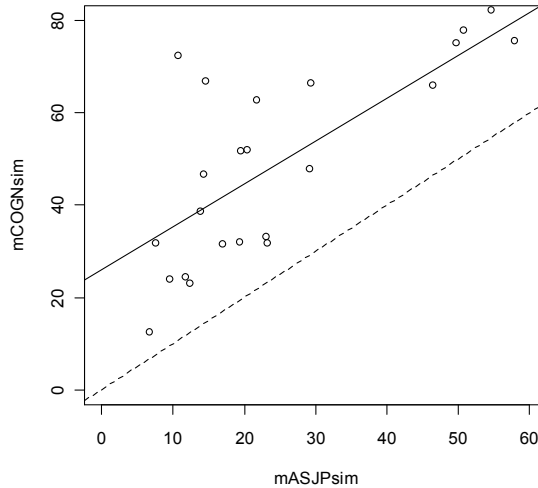
Figure 2. Scatter-plot of mCOGNSim against mASJPSim
