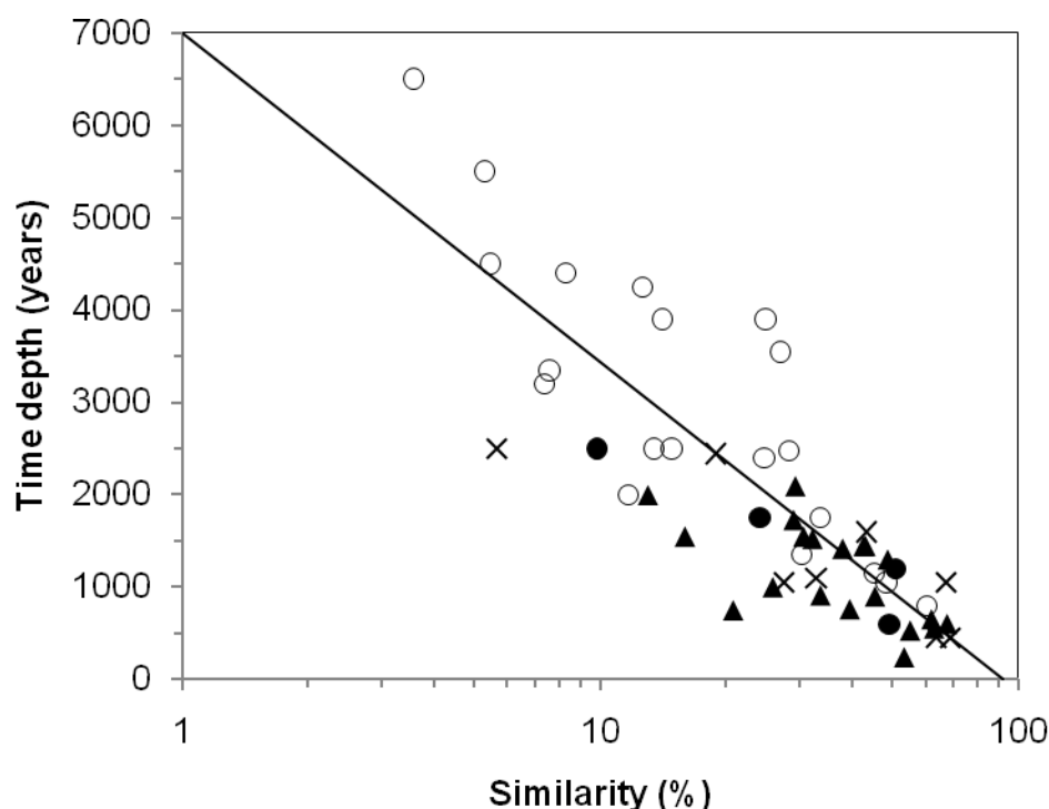
Fig. 2. Time depth ( t ) as a function of similarity ( s ) with regression line; dates are archaeological (open circles), archaeological and historical (filled circles), historical (triangles), and epigraphic (Xs).
